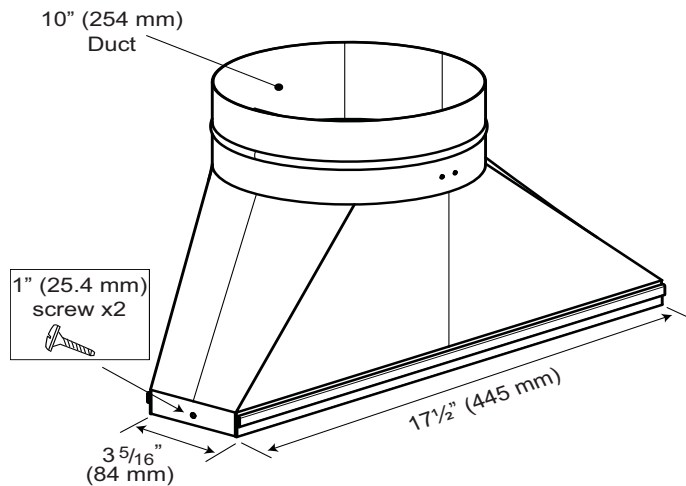
Figure 2: Transition Dimensions
