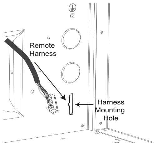
Figure 14: Remote Harness Mounting Hole
