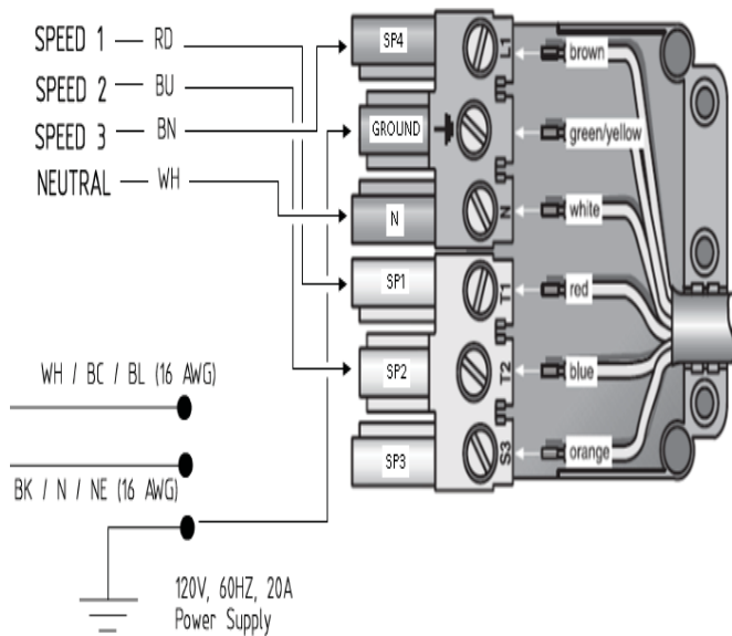
Figure 9: Wiring the Hood with a Remote Blower
