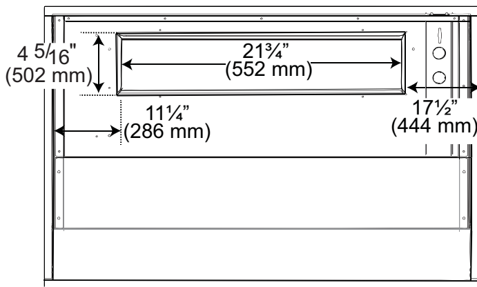
Figure 3: Transition Cutout
