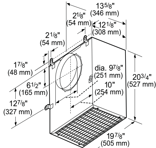
Figure 8: VTR1330E Remote Blower
