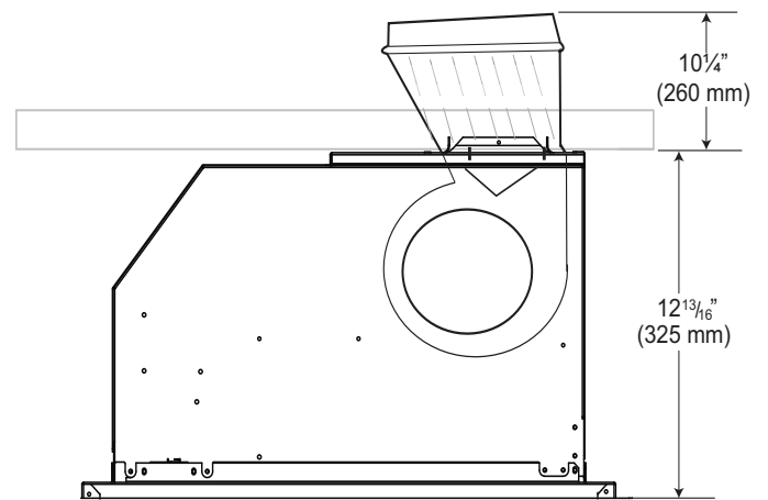
Figure 4: Transition Centerline
