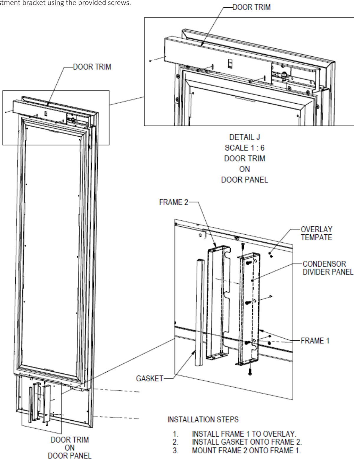
DETAIL K SCALE 1 : 4
