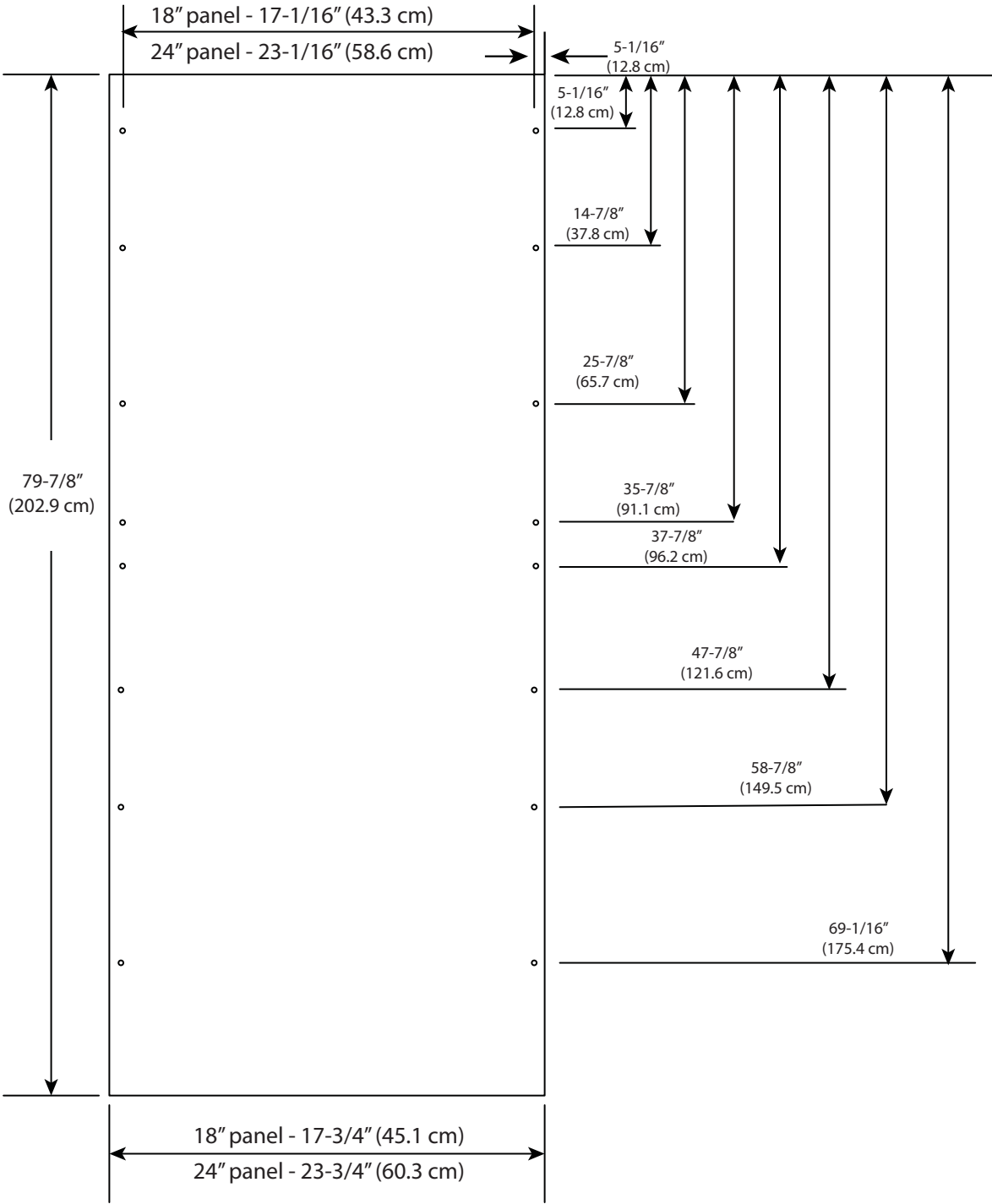
Custom Panel - hole locations
