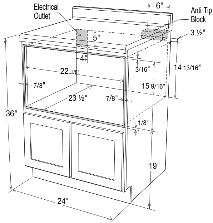
Cabinet Dimensions
